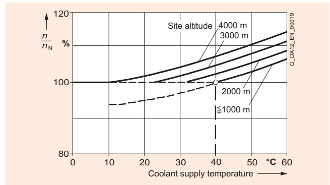
Speed deviations as a function of the site altitude and the coolant supply temperature for DC motors.
