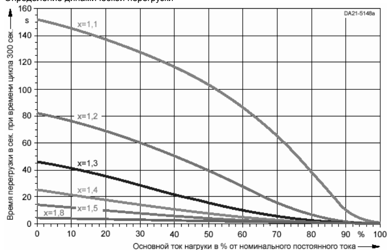
Рис. 5/20 6RA7090-6KV62 1000 A/4Q/690 V, 6RA7088-6LV62 950 A/4Q/830 V
