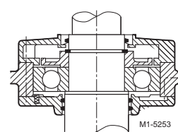
Fig. 7 Drive-end bearing Drive-end bearing Non-drive end bearing
