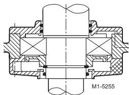
Fig. 7 Drive-end bearing Drive-end bearing Non-drive end bearing
