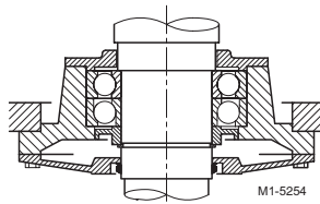
Fig. 7 Drive-end bearing Drive-end bearing Non-drive end bearing
